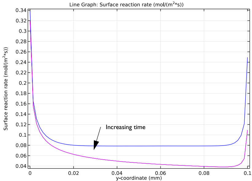
Figure 5: Surface reaction rate at the active surface. The largest reaction rate is obtained initially and is at the edges of the active surface. The reaction process almost reaches steady state at 0.5 s.
